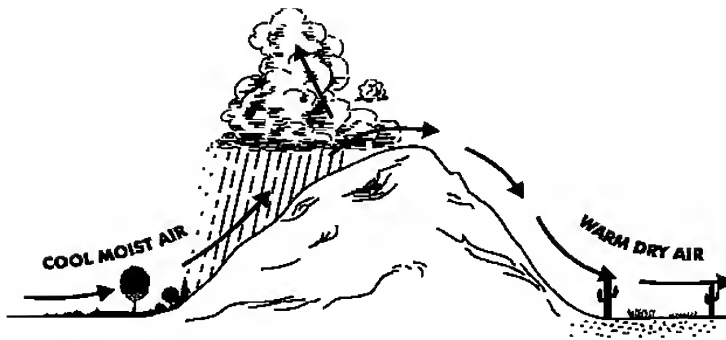
OROGRAPHIC UPLIFT
